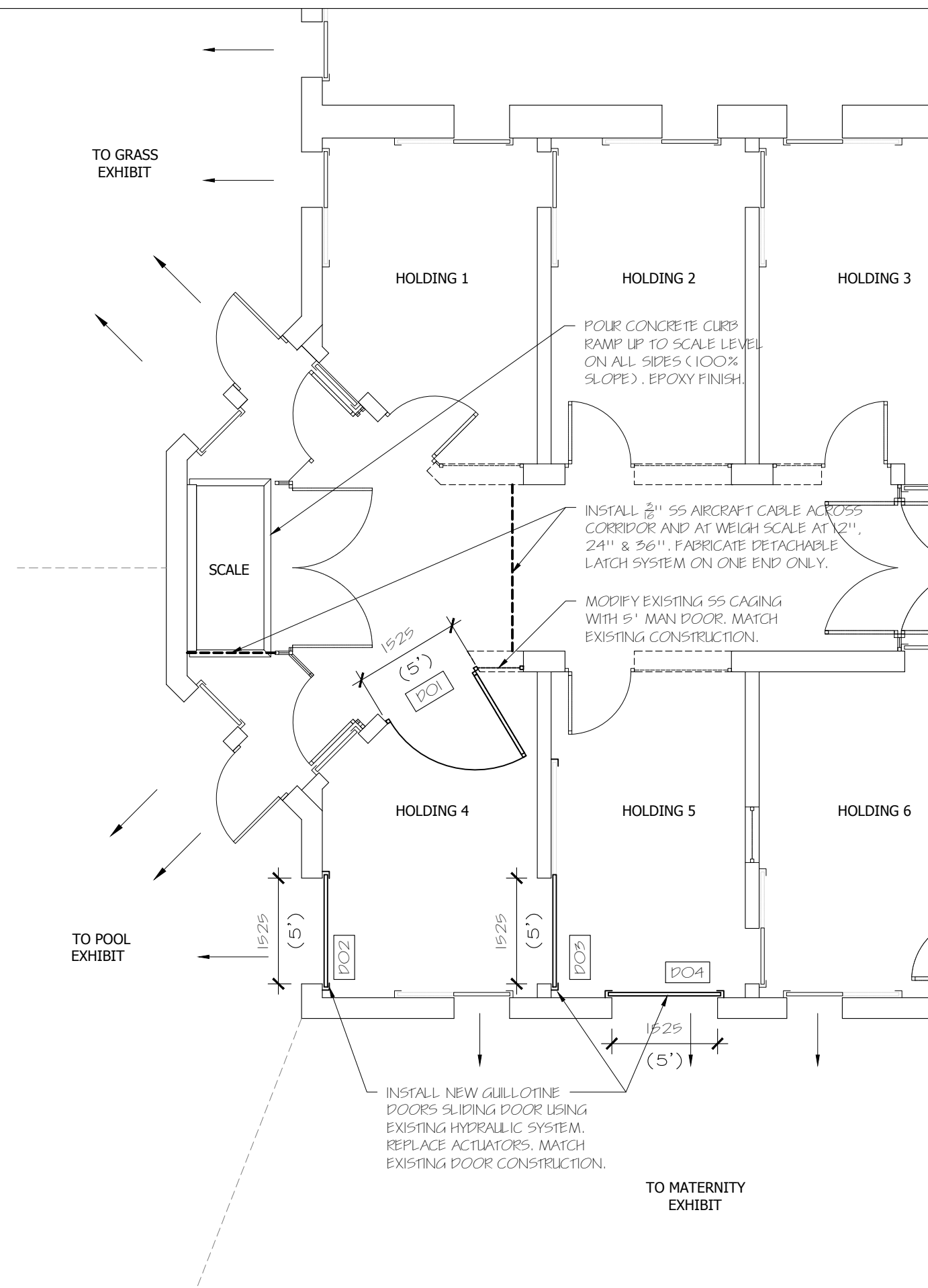
2 PROPOSED FLOOR PLAN Scale: 1:100
